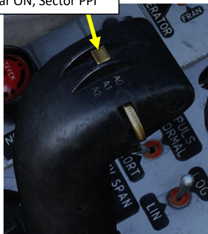
Radar Mode Selector A1: Radar ON, Sector PPI
