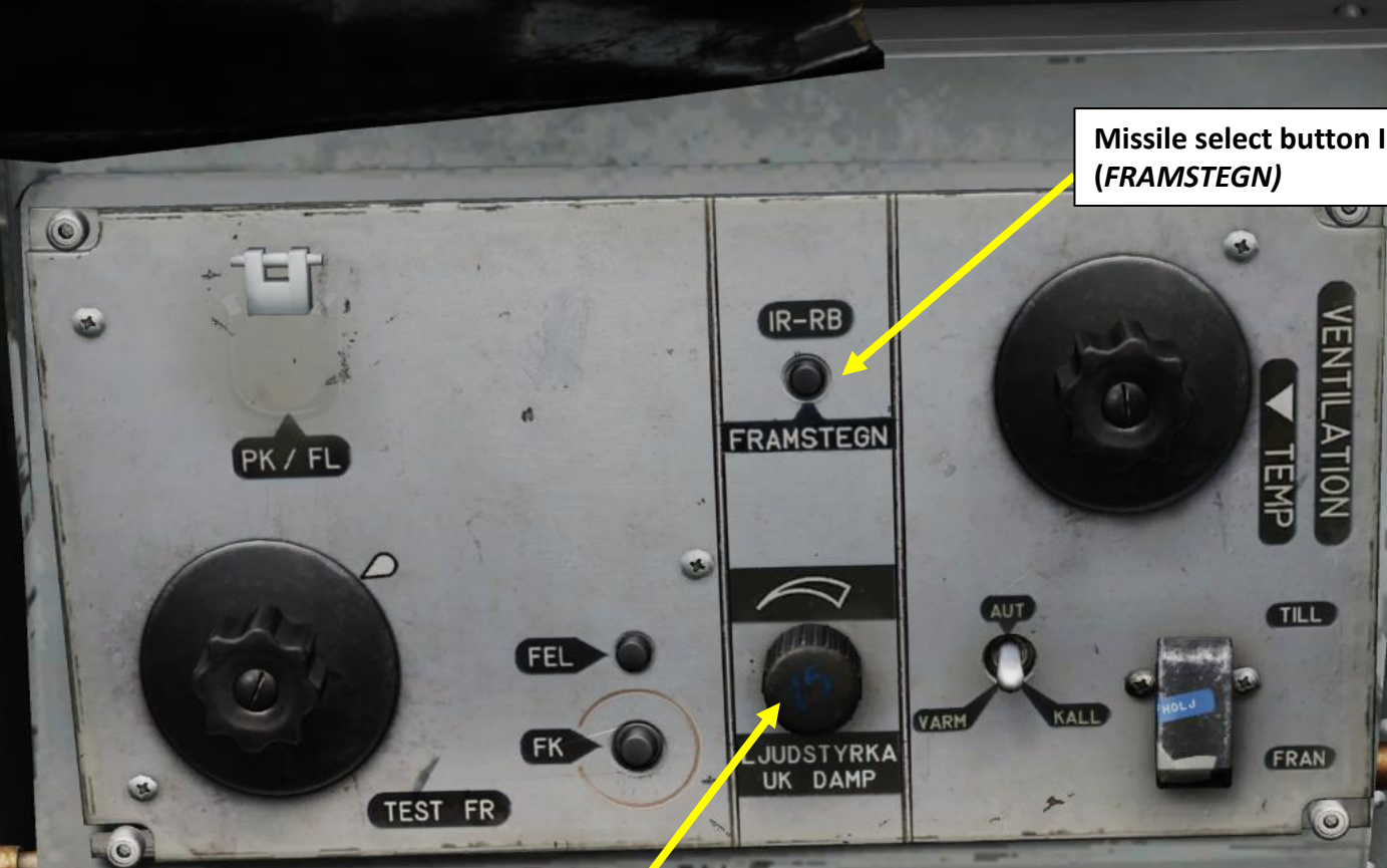
Sidewinder Missile Tone / Radar Warning Receiver Volume Control (Ljudstyrka Uk-Dämp)
