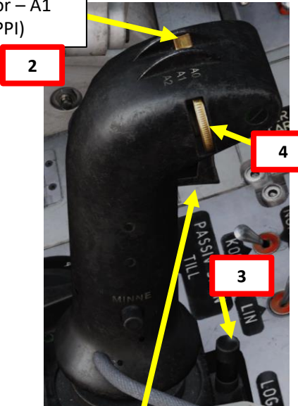
Radar Fix Trigger • T0: Neutral • T1: First trigger detent • TV: Second trigger detent
