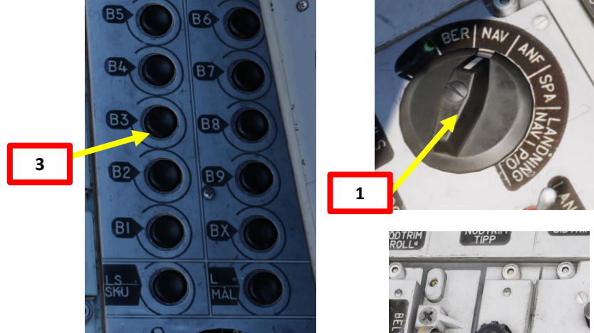
Radar Mode Selector – A1 (Wide Search with PPI) 4
